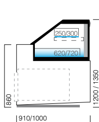
VDS - VD / VD 2P vitruina display case 3H1 (+1... +10 °C) 3M1 (-1... +5 °C) 3M2 (-1... +7 °C) 3S (+13... +15 °C) DIM. (b) 937 | 1250 | 1562 1875 | 2500 | 3125 | 3750 CER45 | CER90 CIR45 | CIR90
