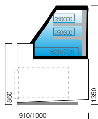
VDS - VD R2P vitruina display case 3H1 (+1... +10 °C) DIM. (b) 937 | 1250 | 1562 1875 | 2500 | 3125 | 3750
