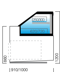
VDS - VD R1P vitruina display case 3M2 (-1... +7 °C) DIM. (b) 937 | 1250 | 1562 1875 | 2500 | 3125 | 3750 CER45 | CER90 CIR45 | CIR90
