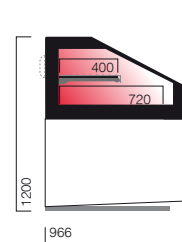
VMDS Aq grab & go aquecido heated grab & go DIM. 937 | 1250
