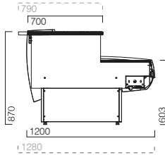
CCX caixa support counter caisse caja
