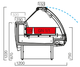
VCBM VC-CH banho-maria bain-marie baño maría
